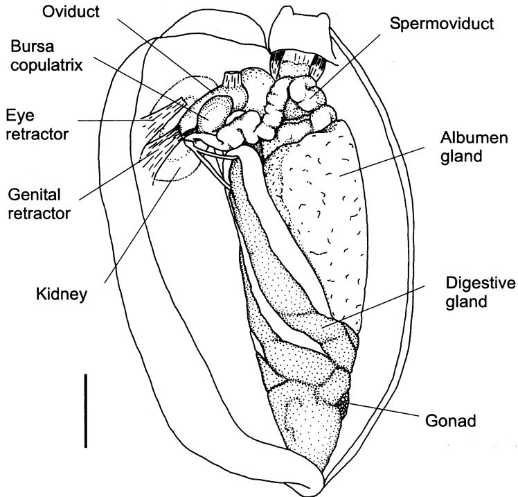
Fig. 2: Internal morphology of the sinistral specimen. Scale bar = 10 mm.
